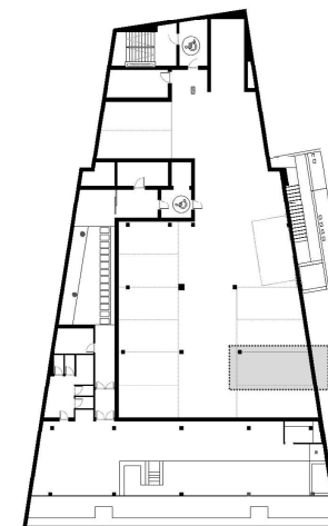
GARAGE floor -3
