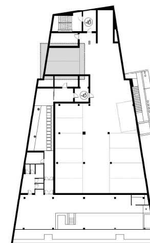
GARAGE floor -3
